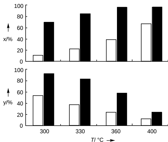
Figure 1. The effect of temperature on the conversion of 1 (x) and selectivity for N-methylated products (y) in the gas phase (white bars) and the supercritical phase, P = 8.2 MPa, (black bars) in the methylation of 1 over the Cs-P-Si catalyst. Conditions: W/F = 25 g h mol -1 , CH 3 OH/amine = 10.8/1.
